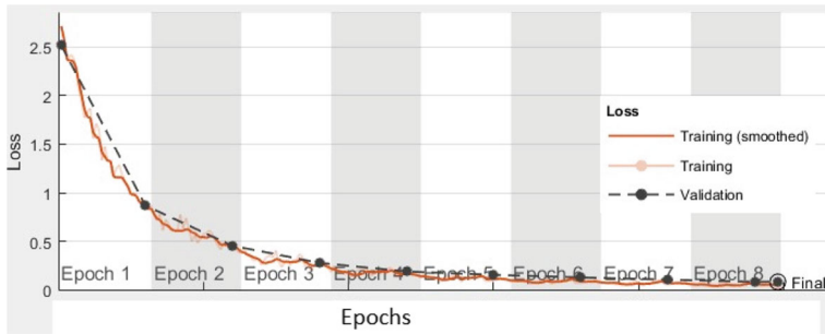
Fig. 7 CNN loss curve for the public dataset
