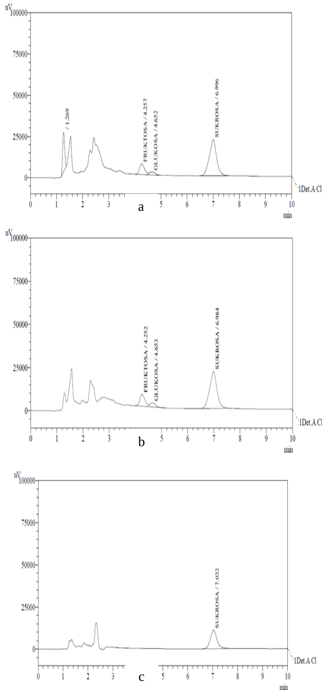
Fig 2. Simple sugar content chromatogram on a. Palm Sugar, b. Coconut Sugar, c. Sugar Cane
