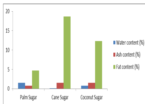
Fig 1. Water content, ash content and fat content in palm sugar, sugar cane and coconut sugar
