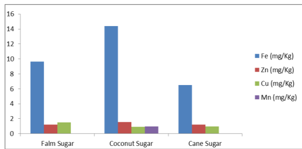
Fig 3. The content of metal minerals in palm sugar, sugar cane and coconut sugar
