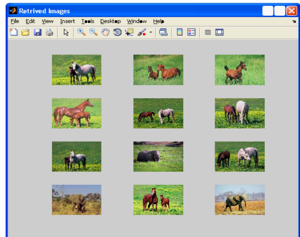
Fig 5: Rerieved iamge
